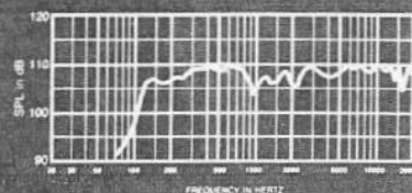
FIGURE 1 MTH-4A Axial Frequency Response Using MTX-4 Electronics Unit (1 watt/1 meter into MB section)
